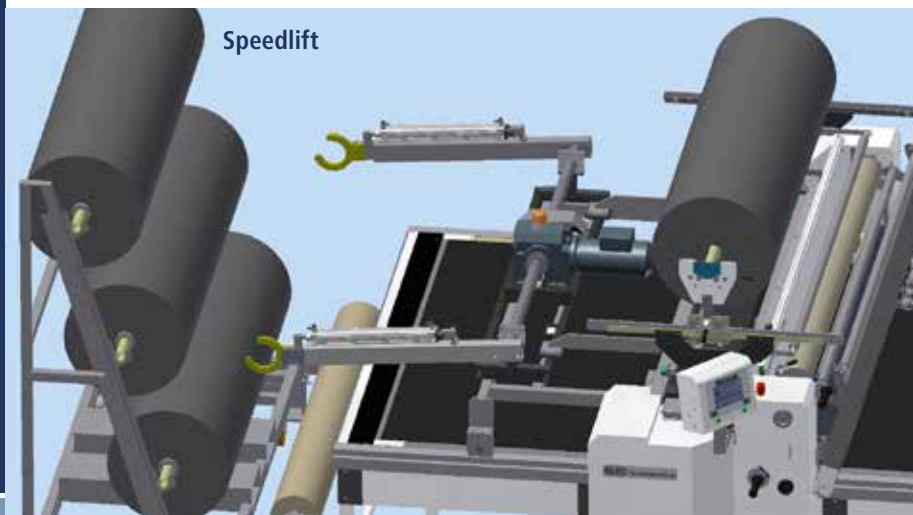
Loading unit-inclined lift for a machine with cradle
